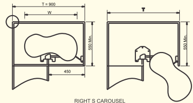
RIGHT S-CAROUSEL
