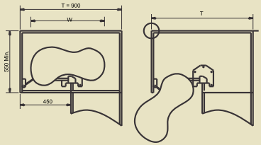
LEFT S-CAROUSEL
